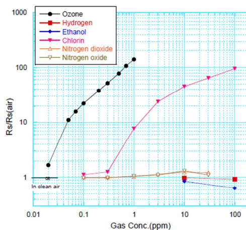
Fig. 3 Sensitivity characteristics
