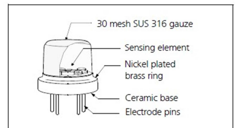
Fig2 .Structure
