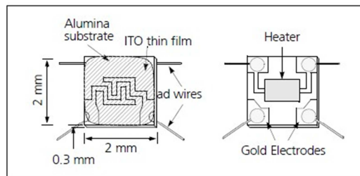
Fig 1. Sensing Elements
